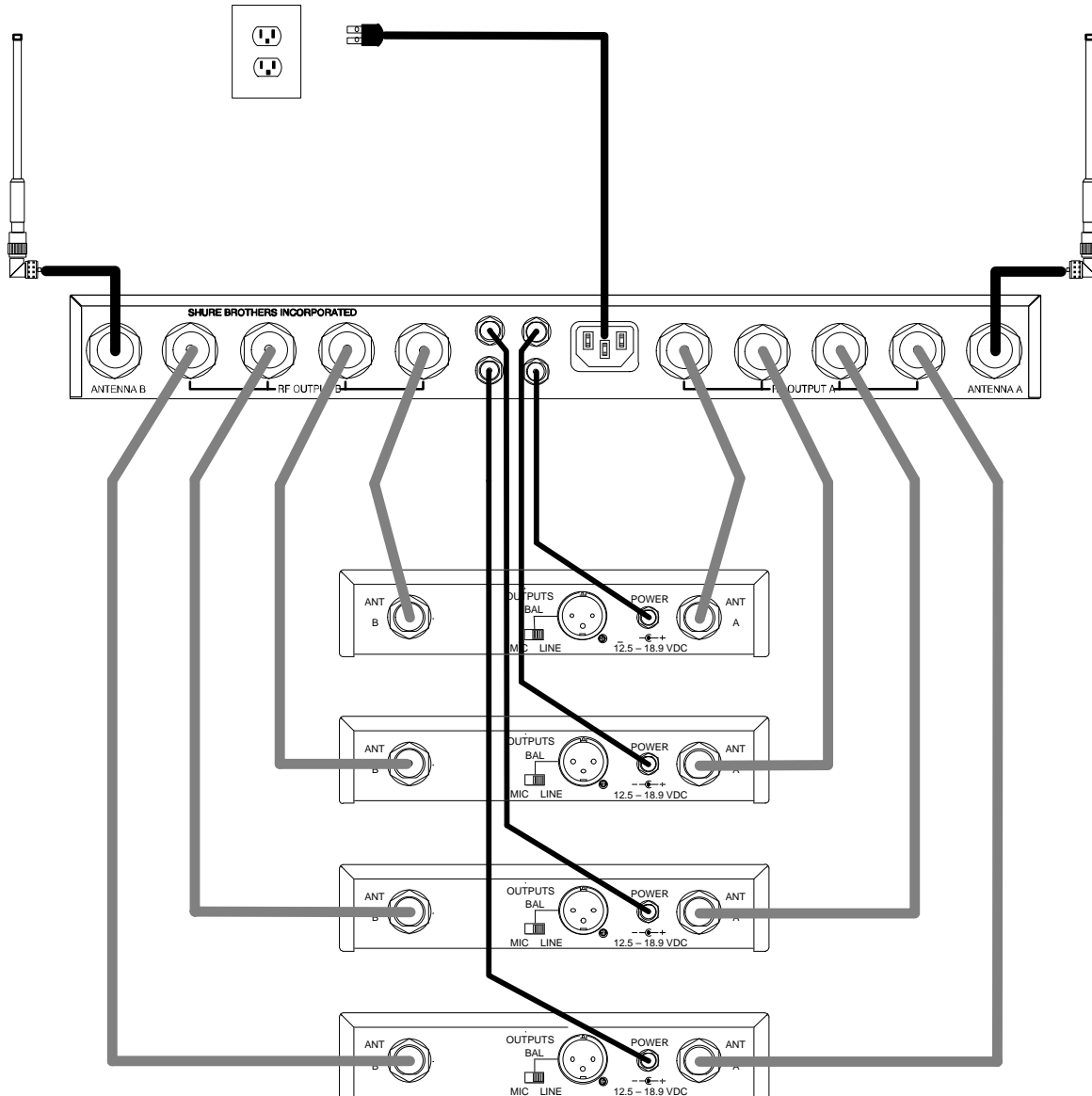
WA405 SETUP FIGURE 7
