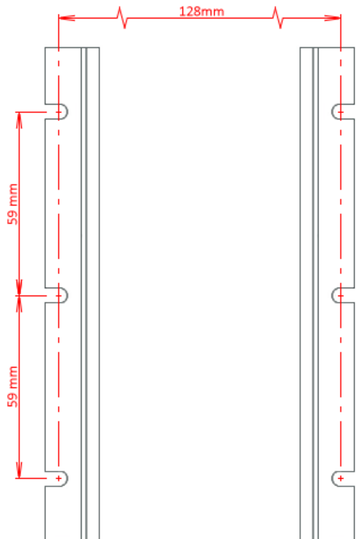
Fig 1: Mounting Bracket Fixing Positions Drawing not to scale
