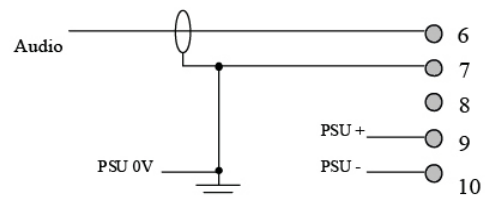
Fig. 1 – Meter, Audio & Power Connections
