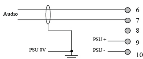
Fig. 1 – Meter, Audio & Power Connections
