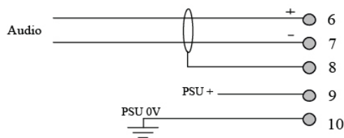
Balanced Input, Single Rail Power
