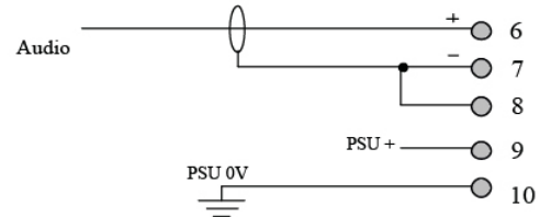
Un-balanced Input, Single Rail Power
