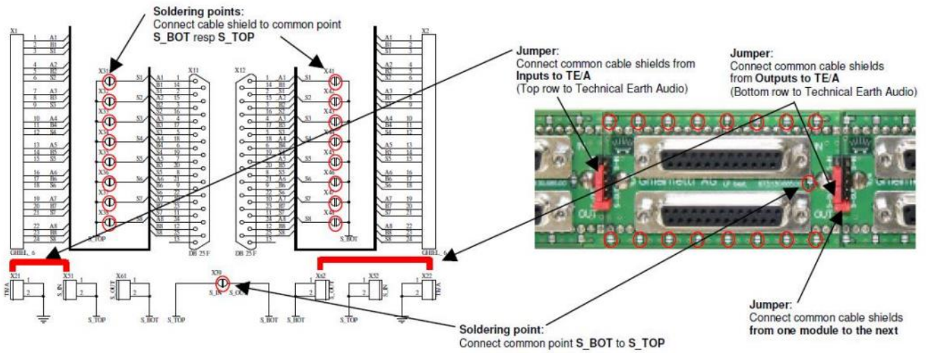
CSF 1x48 AV 3/1 D25Sffcs 19", 1RU, incl. 6 D-Sub 25-pole modules for common-shield connecting facilities 673.113.553.47
