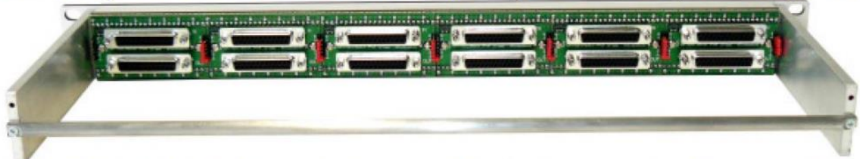
CSF 1x48 AV 3/1 D25Sffcs 19", 1RU, incl. 6 D-Sub 25-pole modules for common-shield connecting facilities 673.113.553.47
