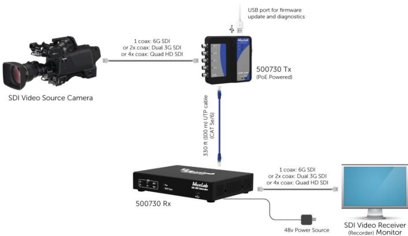
Figure 1: System Overview
