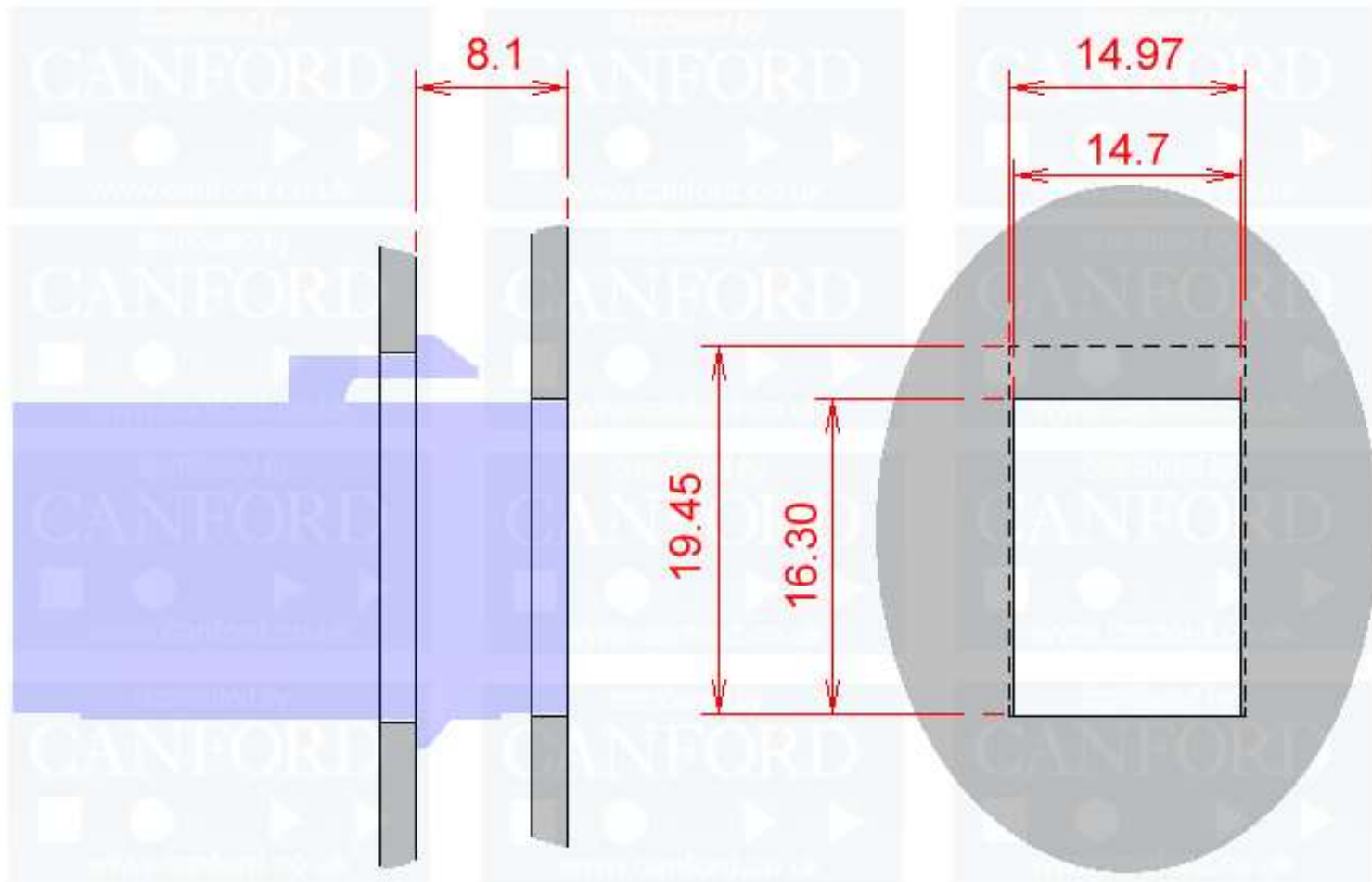
Section through panel (All dimensions - mm)
