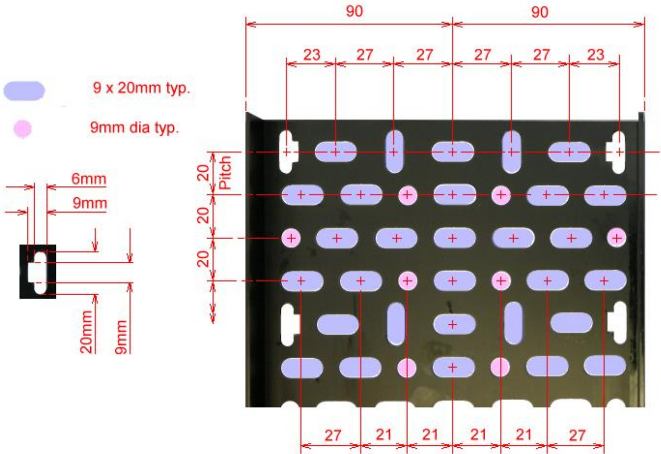
Canford plastic cable tray 180mm x 17mm x 2.5mm thk Supplied in 2m lengths
