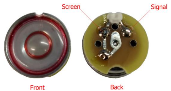
27-802 Mic Capsule - Post Nov 2021
