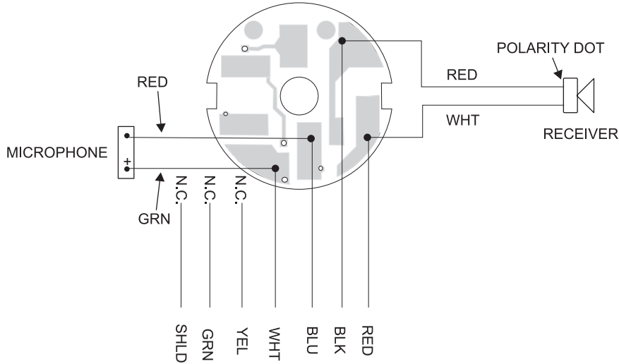
Wiring Diagram
