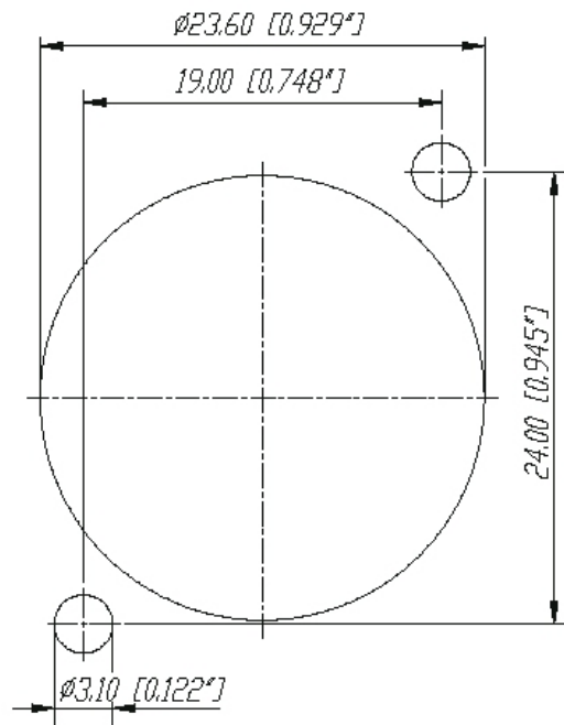
Panel cut out (rear side)
