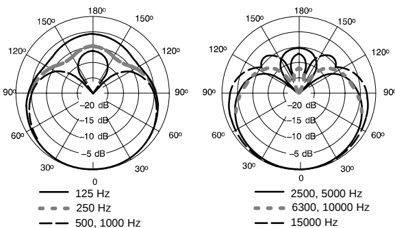
TYPICAL POLAR PATTERN FIGURE 3
