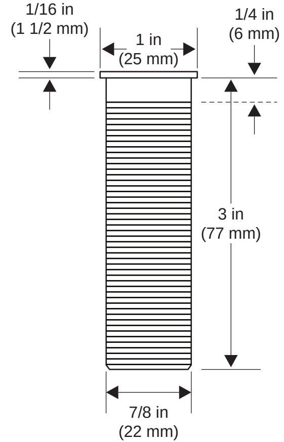
31A2165 Mounting Tube
