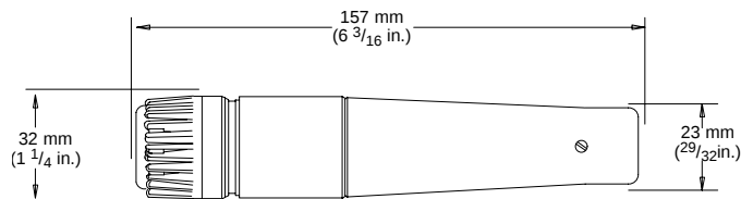
DIMENSIONS FIGURE 5
